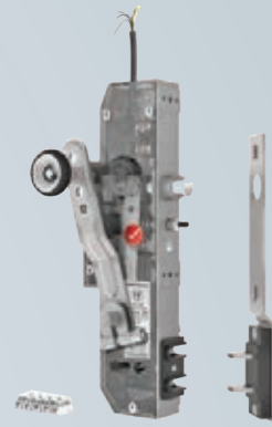
DOUBLE SECURED PASSENGER ELEVATOR SEMI AUTOMATIC DOOR LOCK
